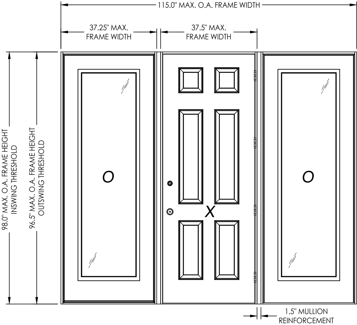
OPAQUE SINGLE DOOR w/ SIDELITES
