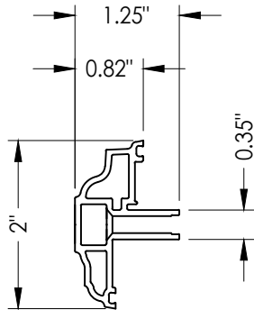
23 INTERIOR LITE FRAME ODL
