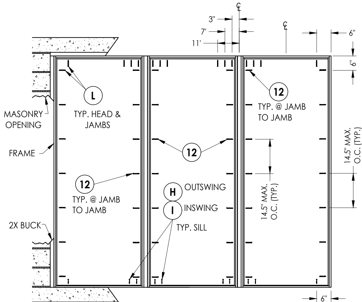
FRAME ANCHORING Masonry 2X buck construction
